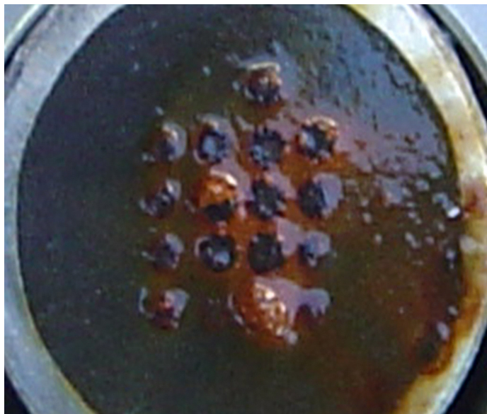
Figure 7. Appearance of the CS 1008 probe immediately after removal from the simulated seawater, after the corrosion rate measurement.
